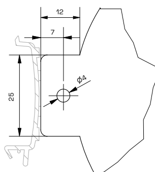
Die-cutting pin dimensions
